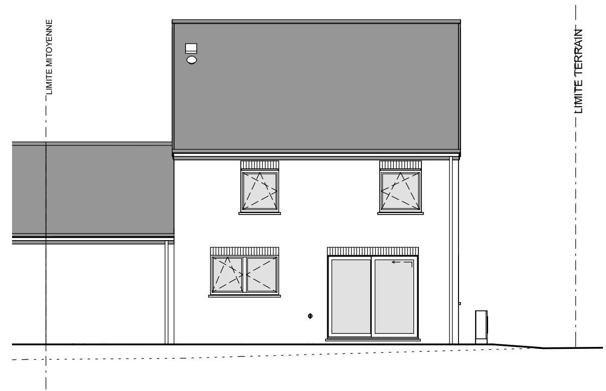
FACADE ARRIERE
